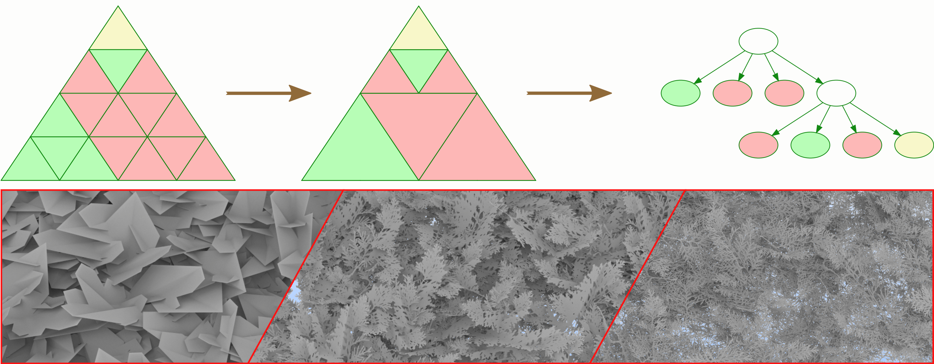
Figure 4: Hardware accelerated ray-tracing process can struggle with partially-transparent triangle meshes, but by leveraging a structure known as opacity micromaps that issue is alleviated. In this work, this construct is extended with a novel compression scheme.
