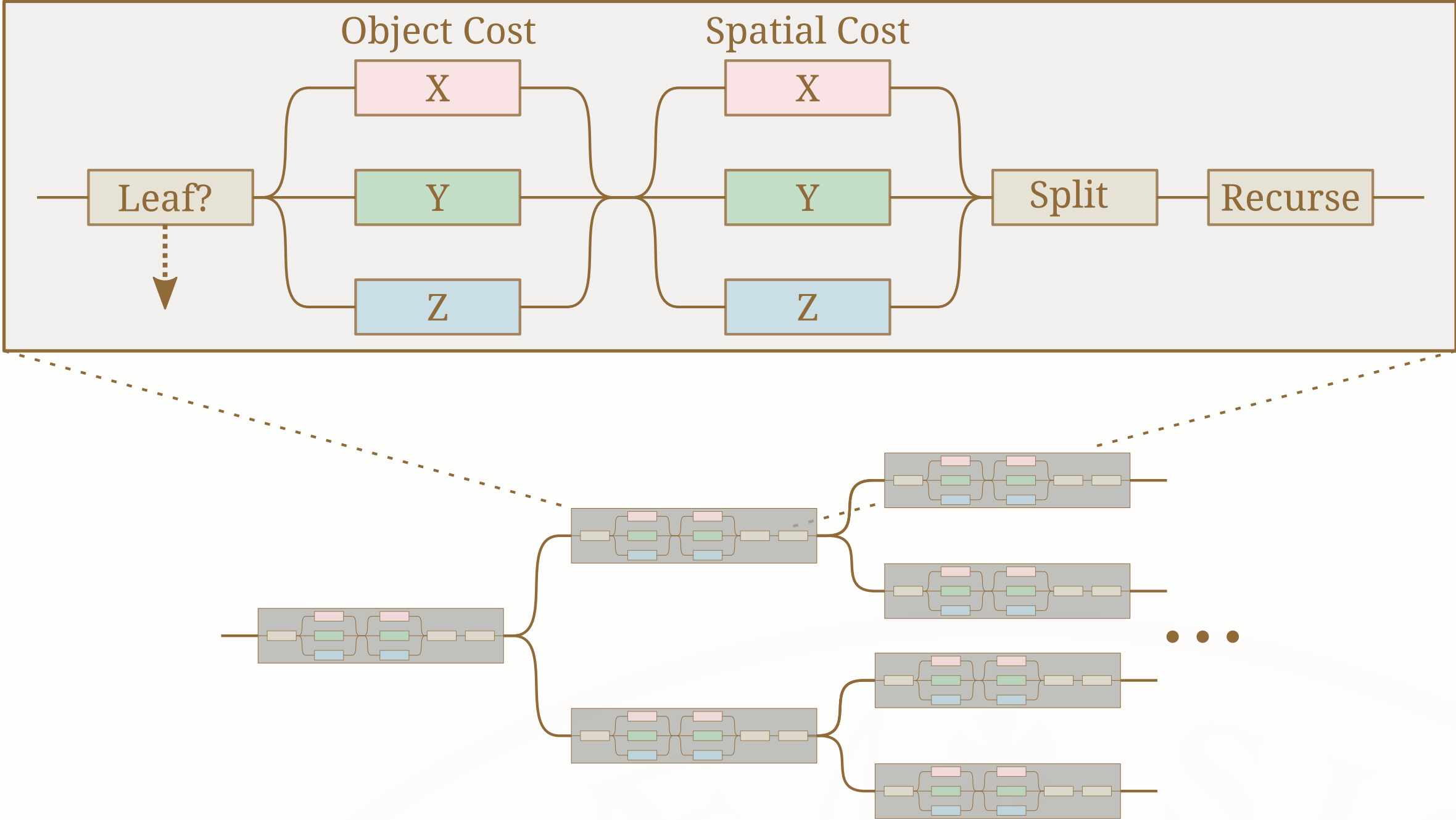
Figure 5: A small but important detail of rendering is the construction of the BVH, here, the parallelization of BVH construction is done with a simple and straightforward application of OpenMP .
