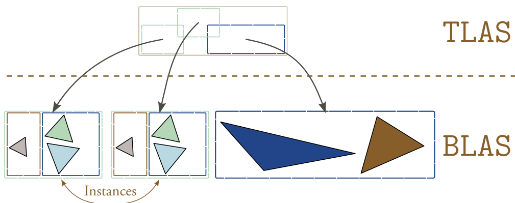
Figure 31: The hardware version of the acceleration structure consists of two levels: The Top Level Accelerations Structure (TLAS), and the Bottom Level Acceleration Structure (BLAS). This organization both enables high-performance ray-tracing and features such as cheap replication of objects that are used multiple times, i.e., instances .
