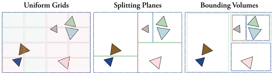
Figure 22: Schematic illustration of three common acceleration structures and the elements they use in their construction. Uniform Grids ( left ) store the geometry in uniformly sized cells. Here visualized with red for cells with overlapping geometry, and green for empty cells. Rather than cells, Kd-trees ( middle ) uses splitting planes to hierarchically separate geometry, and instead of planes, bounding volume hierarchies uses nested boxes to create a hierarchy to contain the objects.
