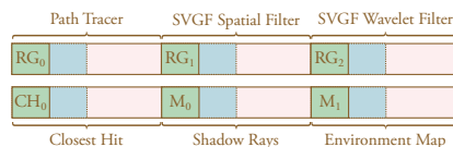
Figure 2: The Shader Binding Table (SBT) control both the rendering and filtering: The first RayGen-shader performs the primary rendering, and optionally, the temporal filtering, whereas the remainder perform the actual SVGF passes, the spatial and à trous wavelet filters.
