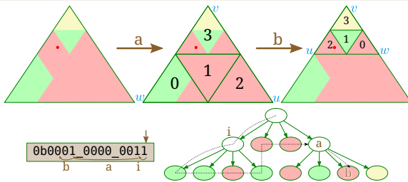
Figure 2: Bitwise comparison of the original opacity micromap and the tree from the above example.
