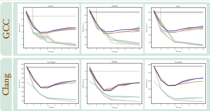
Figure 4: Beyond OpenMP tasking from figure 2, the object and spatial axis searches may also be accelerated, as each axis is independent. However, there are numerous ways to use OpenMP when tasking is already being applied elsewhere. Thus, the following OpenMP #pragma variants were applied to these to loop to find the best way. Thus, in total we have 8 different variations: With or without tasking, and 4 different ways to accelerate the inner axis for-loops.
