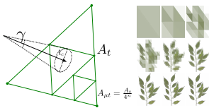
Figure 4: Well defined mipmap constructs for micromaps.
