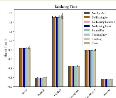
Figure 5: Estimated rendering times for each scene and variant.
