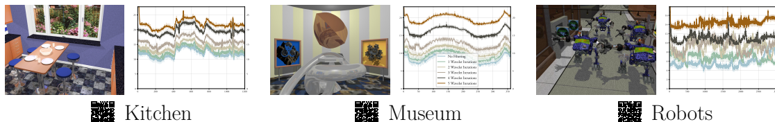
Figure 4: The BART [1] scenes and associated framerate results in milliseconds (ms) for each frame of the animation with either no filtering, or up to 5 iterations of the à trous wavelet filtering. Additionally, this work includes a gLTF conversion of the original AFF scenes, available through the QR-codes, albeit limited to linear animations for the time being.
